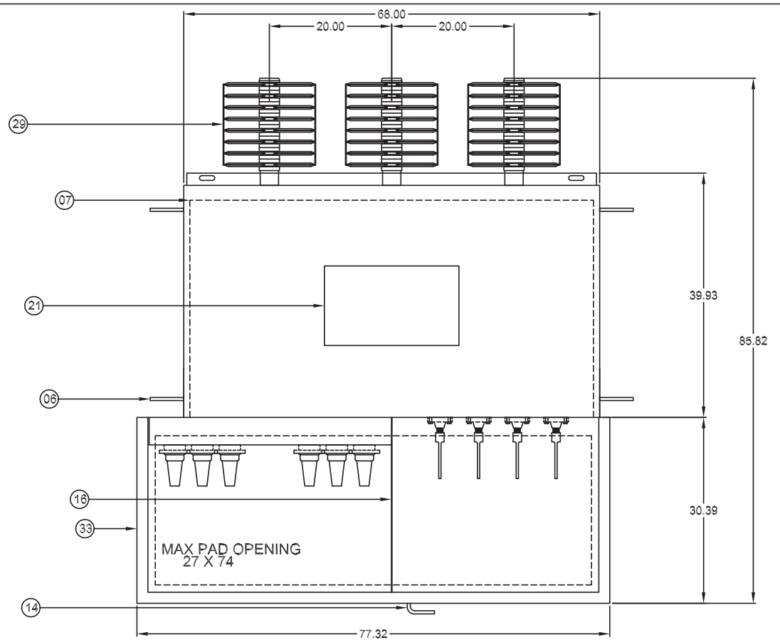
TOP VIEW WITH CABINET COVER REMOVED
