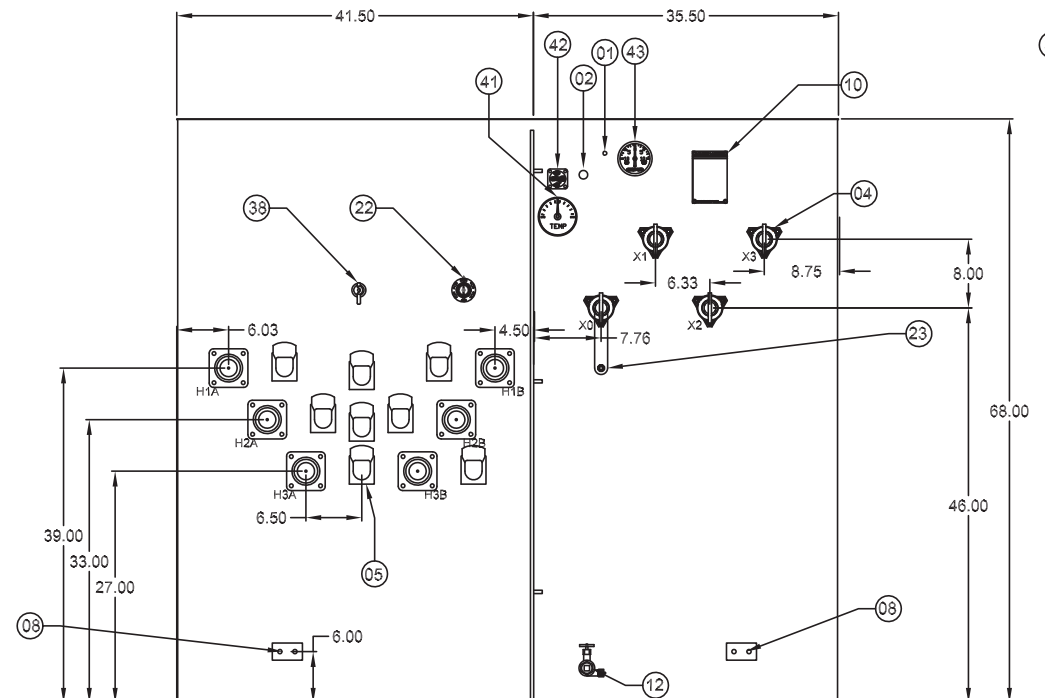
FRONT VIEW WITH CABINET REMOVED
