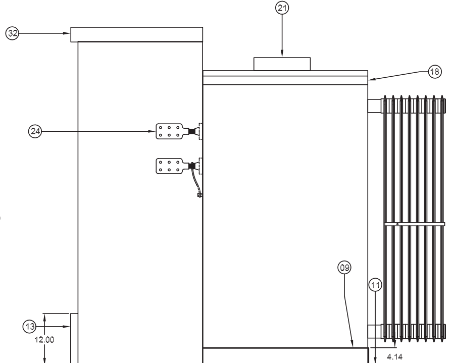
SIDE VIEW WITH CABINET DOORS AND SIDES REMOVED
